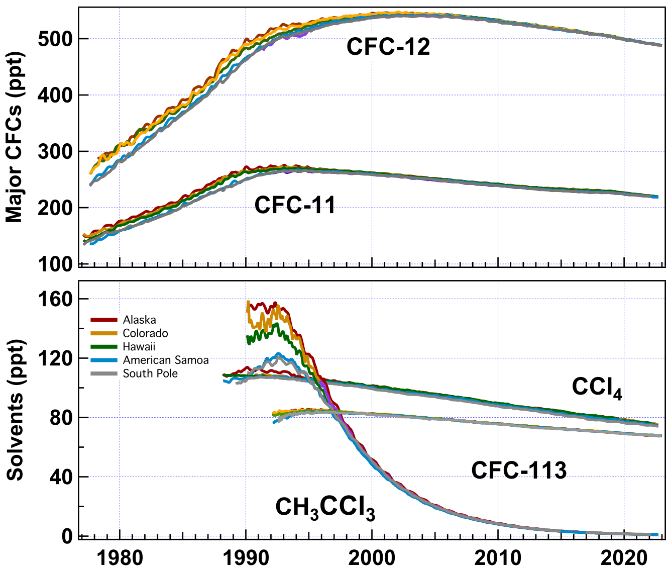
Atmospheric abundances (in parts per trillion, ppt) of the main chlorine-containing gases regulated by the Montreal Protocol. Measurements are from four NOAA atmospheric baseline observatories and Niwot Ridge, Colorado, NOAA Global Monitoring Laboratory.
